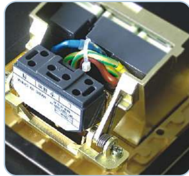
Terminal block code: FLS-TB-001 Fast connection terminal
